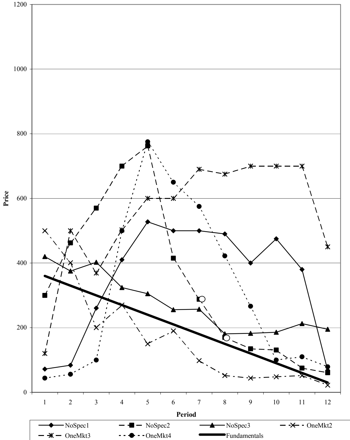
Figure 1: Time Series of Median Transaction Prices by Period: NoSpec and 12-Period OneMarket Sessions
