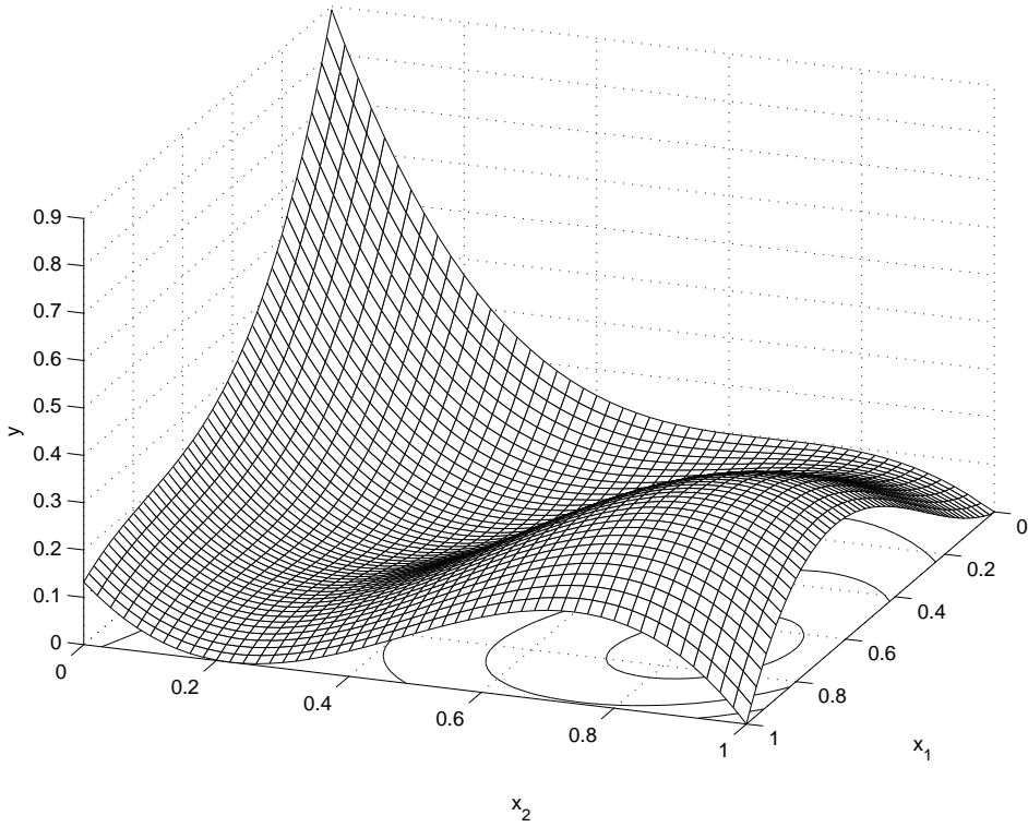
Figure 2: Nonnegative polynomial of Example 2.1 with nonnegativity-constraint.
