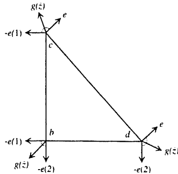
Fig. 3. Stationary points of g on \text{bd}(\bar{\mathcal{N}}(\bar{t}) \cap \mathbb{R}_+^2) .
