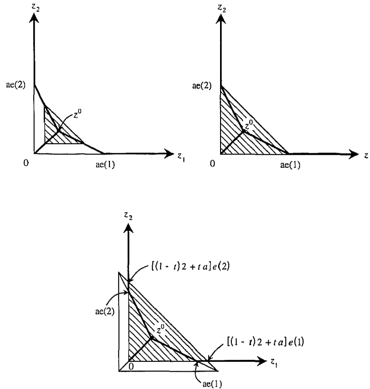
Fig. 1. The subset \mathcal{N}(t) \cap \mathbb{R}_+^2 for t = \frac{1}{2}, 1 , resp. \frac{1}{2} , given z^0 = (1, 1)^T and a = 3 .
