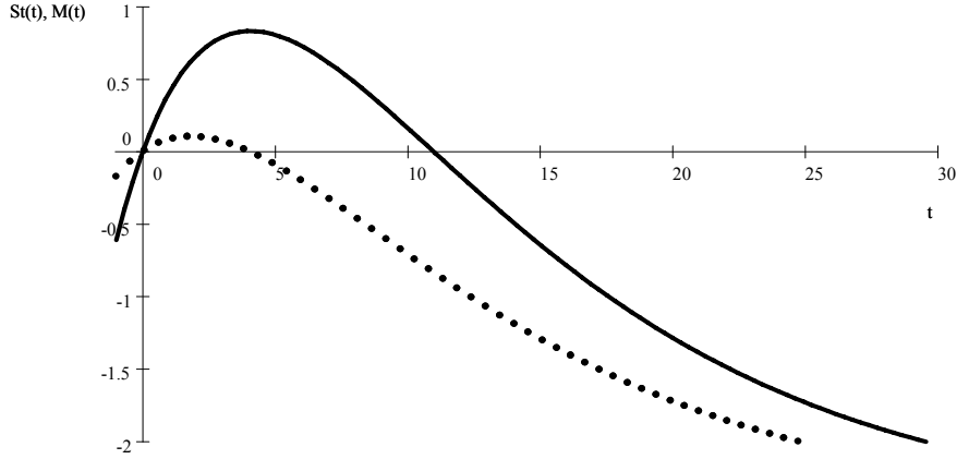
Figure 3: Graphs of St(t) and M(t) for case \alpha\lambda > 2r . Parameter values are
