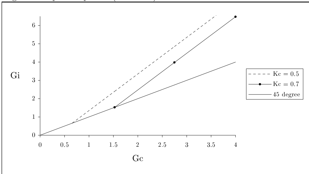
Figure 5: Asymmetry in G ( \mu = 0.5 )
