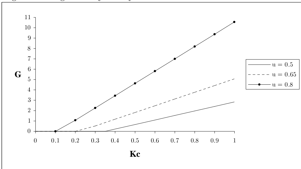
Figure 3: Recognition asymmetry in favor of incumbent
