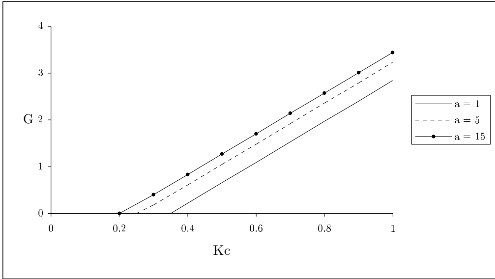
Figure 4: Cost of access asymmetry in favor of incumbent
