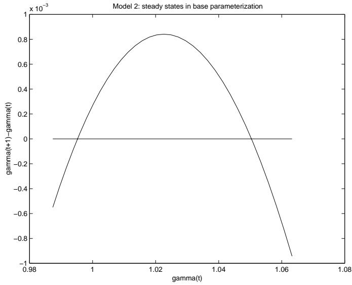
Figure 2: This figure shows the multiple steady states in model 2 in its base parameterization, plotting \gamma_{t+1} - \gamma_t versus \gamma_t . Check the intersections with the horizontal line at zero. The high growth steady state is approximately at \bar{\gamma}_H = 1.05 , whereas the low growth steady state is approximately at \bar{\gamma}_L = 1.00 .
