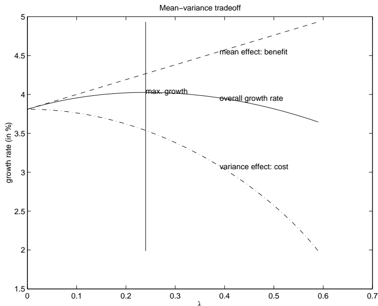
Figure 1: This figure shows the mean-variance tradeoff in model 1. The solid middle line shows the overall growth rate, resulting from mixing the mean effect (straight upper line) with the variance effect (curved lower line). The growth rate is maximized at the value \lambda , which is indicated by a vertical line.
