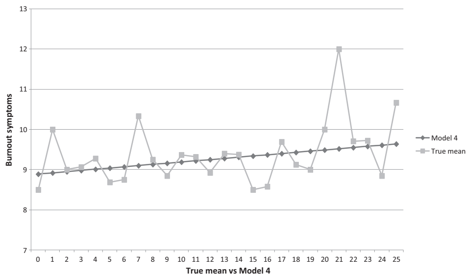
FIG. 2: Mean sum of burnout scores vs estimated mean burnout scores in model 4
