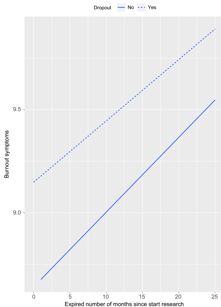
FIG. 1: Regression slopes on the sum of burnout symptoms for dropouts vs nondropouts
