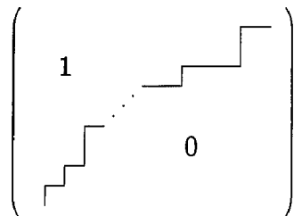
Fig. 1. A \{0,1\} matrix in echelon form.
