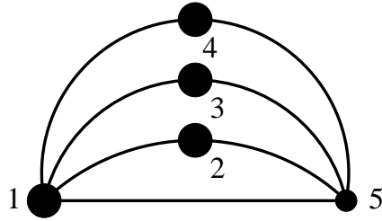
Figure 1: The matroid S_8 is a graft
