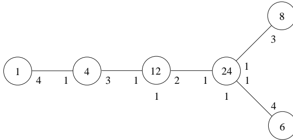
Figure 1: Distance distribution diagram of the flag graph
