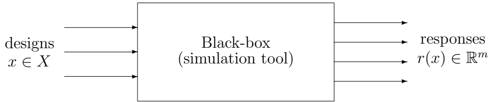
Figure 1: Black-box optimization.
