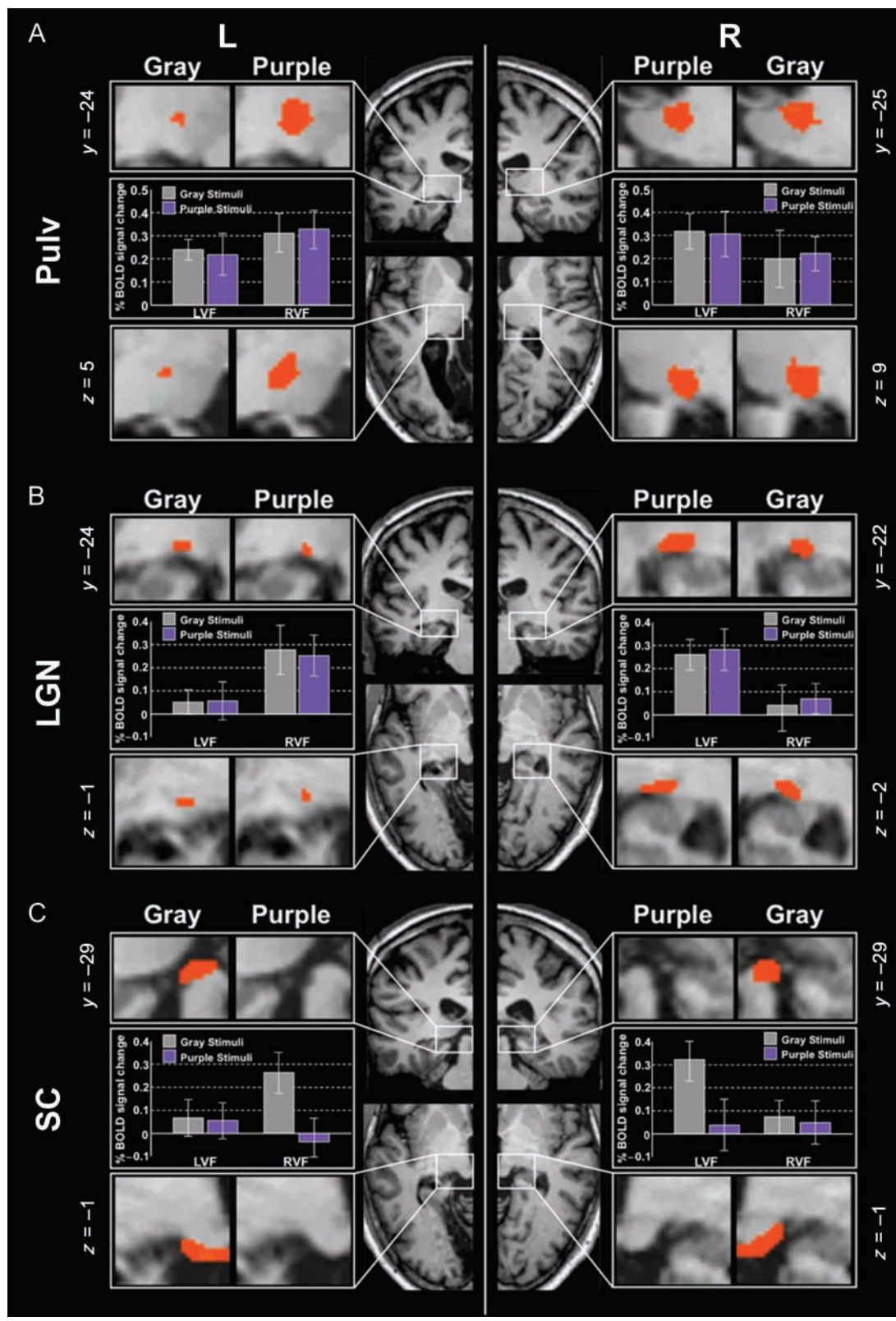
Figure 3. fMRI response to single gray and purple stimuli in subcortical visual structures. Activation maps and mean % of BOLD response from baseline evoked by single gray and purple stimuli in the pulvinar (A), LGN (B), and SC (C). Central panels show T1-weighted anatomical images of G. Y.'s brain in the coronal and transversal planes. Boxes indicate the location of the panels to the left (L) and right (R). Each lateral panel shows the voxels activated within the magnified regions by single gray and purple stimuli separately. The histograms represent the mean % of BOLD signal change ( \pm SEM) for the voxels in the activated cluster as a function of stimulus color and position. Talairach z - and y -coordinates are given. Note the lesion to left V1 visible in transversal slices. BOLD = blood oxygen level dependent; L = left side; LGN = lateral geniculate nucleus; LVF = left visual field; Pulv: pulvinar nucleus; R = right side; RVF = right visual field; SC = superior colliculus.
