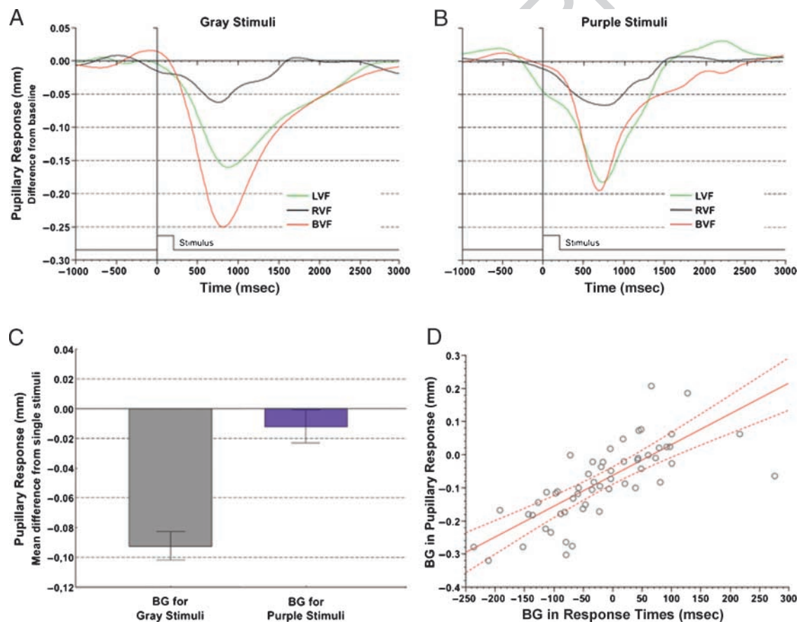
Figure 2. Amplitude and latency of mean pupillary response. (A) Mean pupillary response waveforms during presentation of single LVF, RVF, and BVF gray stimuli. Data are expressed as differences in pupillary diameter from prestimulus baseline. The rectangular pulse trace along the horizontal axis shows the time of stimulus presentation. (B) Mean pupillary response waveforms during presentation of single LVF, RVF, and BVF purple stimuli. (C) Mean differences ( \pm SEM ) in the amplitude of pupillary response between BVF and single LVF stimuli as a function of color (gray and purple). (D) Correlation between the bilateral gain for gray stimuli in RTs data (BVF gray–LVF gray) and the bilateral gain for the same gray stimuli in the amplitude of pupillary response data. The solid red line represents predicted (i.e., fitted) correlation between behavioral and pupillometric measures. The dashed red lines represent 95% confidence limits. BG = bilateral gain; BVF = both visual fields; LVF = left visual field; RVF = right visual field.
