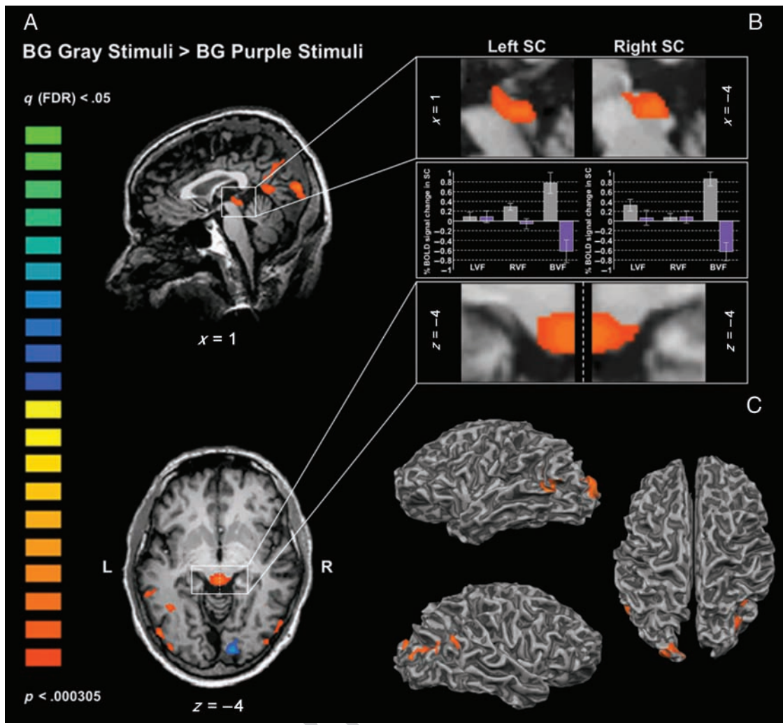
Figure 4. Neural correlates of the bilateral gain. Activation maps and mean % of BOLD response in the SC for the contrast between bilateral gain for gray versus purple stimuli. Areas colored from yellow to red are significantly more activated in the bilateral gain for gray stimuli, whereas areas from blue to green are significantly more activated in the bilateral gain for purple stimuli. Talairach x - and z -coordinates are given. (A) Sagittal and transversal slices of G. Y.'s brain showing significant activations in the left and right SC and in extrastriate visual areas corresponding to higher responses to the condition of bilateral gain for gray stimuli. Boxes indicate magnified regions in the location of the SC shown in B. The ventral portion of the lesion to V1 is also visible. (B) Magnified representation of the activations in the SC and mean % of BOLD signal change ( \pm SEM ) for the voxels in the activated clusters as a function of stimulus color and position. (C) Three-dimensional reconstruction of G. Y.'s brain from lateral and top view showing the occipito-temporal extrastriate areas significantly more activated by the bilateral gain for gray stimuli. The dorsal portion of the lesion to V1 is visible in top view. BG = bilateral gain; BVF = both visual fields; FDR = false discovery rate; LVF = left visual field; RVF = right visual field; SC = superior colliculus.
